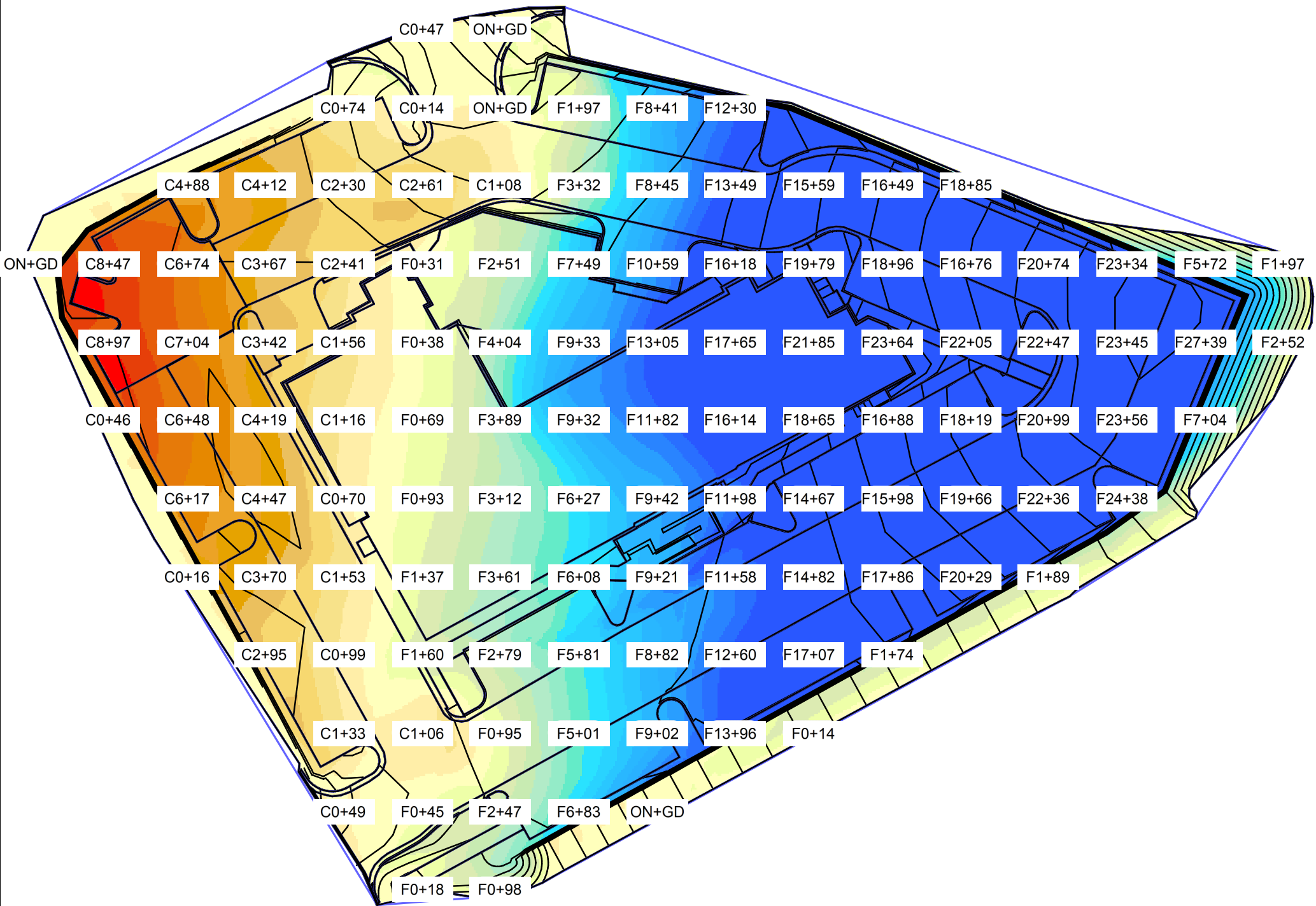
Cut/Fill image
